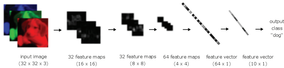
Fig. 7.1 Overview of the CNN used for the image classification task.
